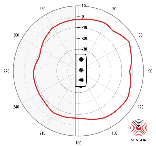
Elevation - 5 GHz
