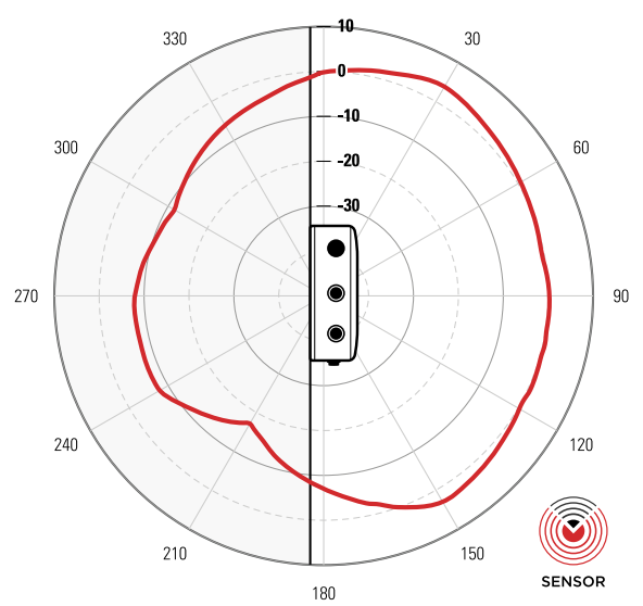
Elevation - 5 GHz
