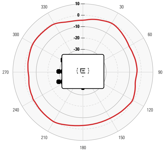
Azimuth - 5 GHz
