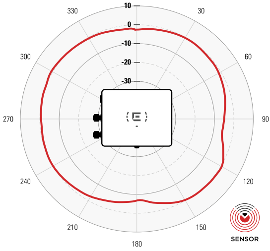
Azimuth - 5 GHz
