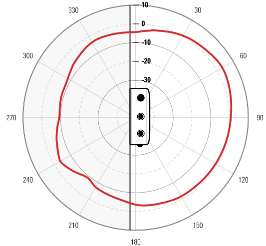
Elevation - 5 GHz
