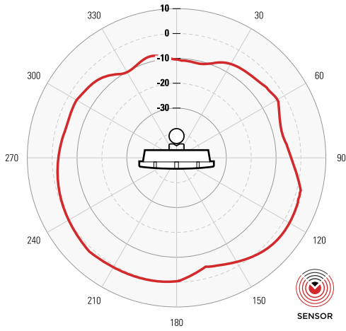
Azimuth — 5GHz
