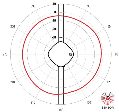
Elevation — 5GHz
