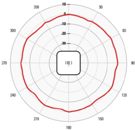
AZIMUTH 5 GHZ
