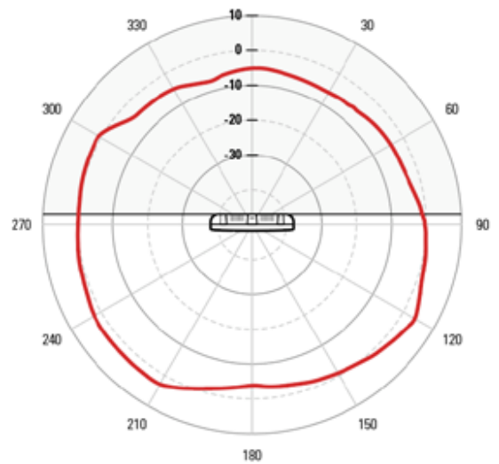
ELEVATION 5 GHZ
