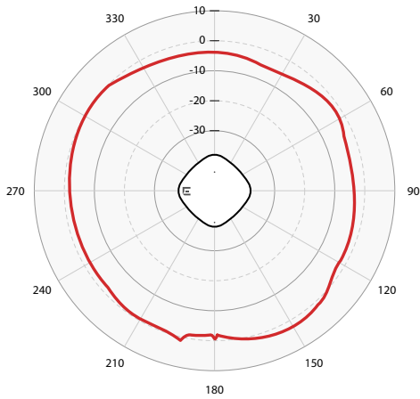
Azimuth - 2.4 GHz
