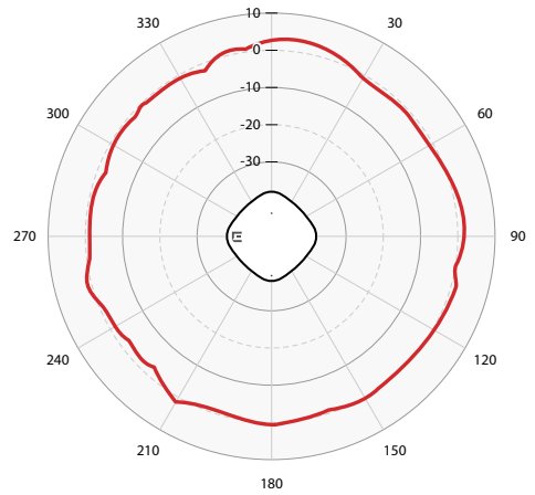
Elevation - 5 GHz
