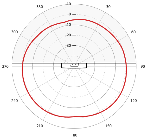
Azimuth - 5 GHz
